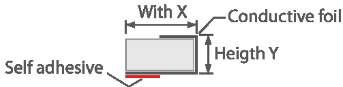
Technical drawing Type 2
