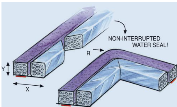
Technical drawing
