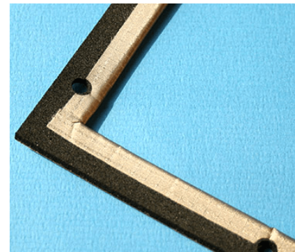
EMC/IP gasket with highly conductive textile (Foil code T)
