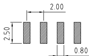
RECOMMENDED PCB LAYOUT (TOLERANCE: ±0.05)
