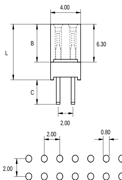
PCB - Layout
